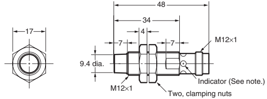
E2A-M12KN05-M1-□□/E2A-S12KN05-M1-□
