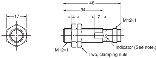
E2A-M12KS02-M1-□□/E2A-S12KS02-M1-□
