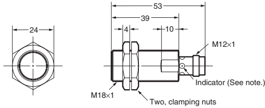
E2A-M18KS05-M1-□□/E2A-S18KS05-M1-□
