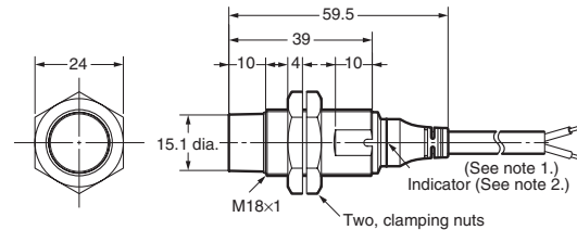
E2A-M18KN10-WP-□□/E2A-S18KN10-WP-□
