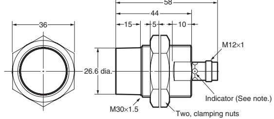
E2A-M30KN18-M1-□□/E2A-S30KN18-M1-□
