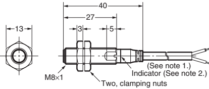
E2A-S08KS01-WP-□□
