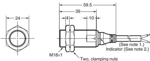
E2A-M18KS05-WP-□□/E2A-S18KS05-WP-□
