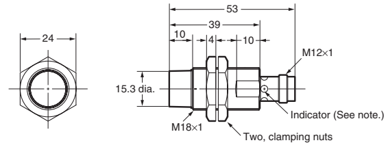
E2A-M18KN10-M1-□□/E2A-S18KN10-M1-□
