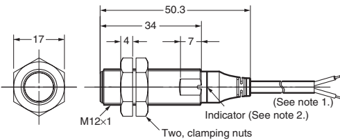
E2A-M12KS02-WP-□□/E2A-S12KS02-WP-□
