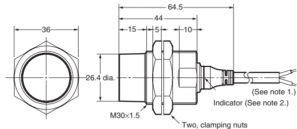
E2A-M30KN18-WP-□□/E2A-S30KN18-WP-□
