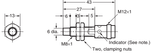
E2A-S08KN02-M1-□□
