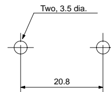
Mounting Holes (for Surface Mounting)
