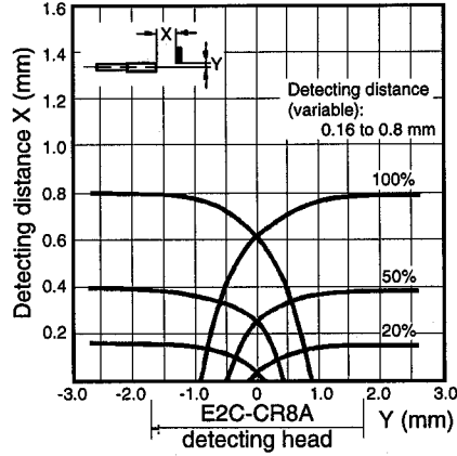
Shielded 3.5 mm dia. sensor E2C-CR8A
